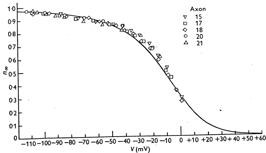
Fig. 5. Abscissa: membrane potential minus resting potential in sea water. Ordinate: experimental measurements of n_\infty calculated from the steady potassium conductance by the relation n_\infty = \sqrt{(g_{K\infty}/\bar{g}_K)} , where \bar{g}_K is the 'maximum' potassium conductance. The smooth curve is drawn according to eqn. (9).
