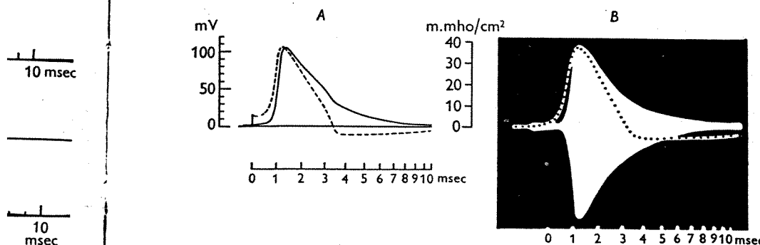
Fig. 16. A , solution of eqn. (26) for initial depolarization of 15 mV at a temperature of 6° C. The broken curve shows the membrane action potential in mV; the continuous curve shows the total membrane conductance ( g_{\text{Na}} + g_{\text{K}} + \bar{g}_l ) as a function of time. B , records of propagated action potential (dotted curve) and conductance change reproduced from Cole & Curtis (1939). The time scales are the same in A and B .
