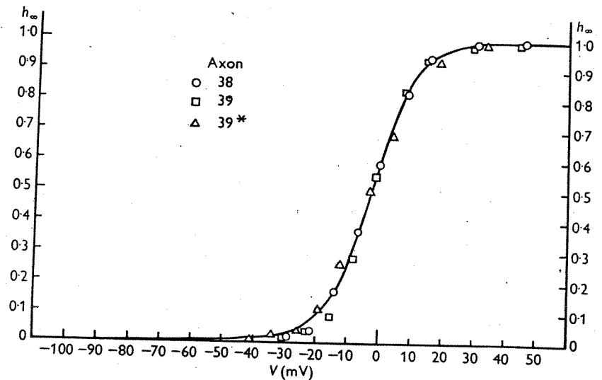
Fig. 10. Steady state relation between h and V . The smooth curve is drawn according to eqn. (25). The experimental points are those given in Table 1 of Hodgkin & Huxley (1952c). Axon 38 (5° C) as measured. Axon 39 (19° C) displaced -1.5 mV. Axon 39* (3° C, fibre in derelict state) displaced -12 mV. The curve gives the fraction of the sodium-carrying system which is readily available, as a function of membrane potential, in the steady state.
