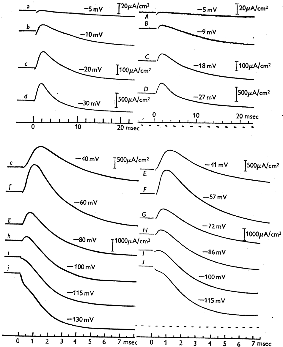
Fig. 11. Left-hand column: time course of membrane current during voltage clamp, calculated for temperature of 4°C from eqn. (26) and subsidiaries and plotted on the same scale as the experimental curves in the right-hand column. Right-hand column: observed time course of membrane currents during voltage clamp. Axon 31 at 4°C; compensated feedback. The time scale changes between d , D and e , E . The current scale changes after b , B ; c , C ; d , D and f , F .
